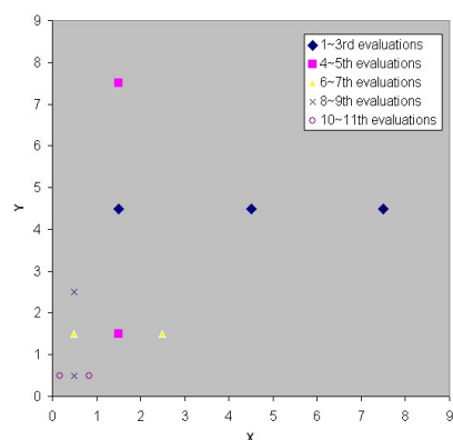
Figure 2: Evaluation trace for GA and GHJ algorithms on a simple 2D function.
