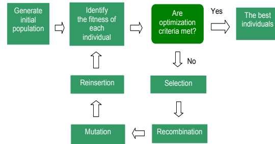
Figure 1: Structure of a single population Genetic Algorithm
