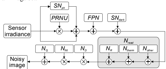
Fig. 1: The derived noise model for image capture in a standard CCD digital video camera.
