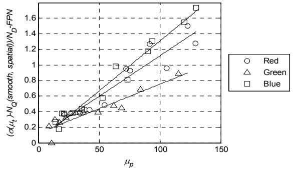
Fig. 5: Measured PRNU for the i400 camera
