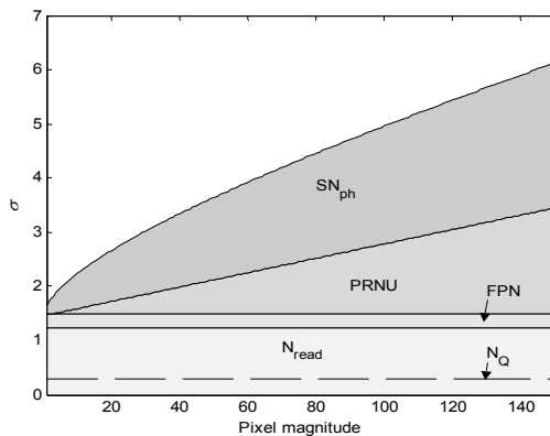
Fig. 7: Relative value of noise components for the blue channel of the i400 CCD camera at 22°C environmental temperature. N_Q denotes the maximum potential quantization noise value, and SN_{dark} is zero.
